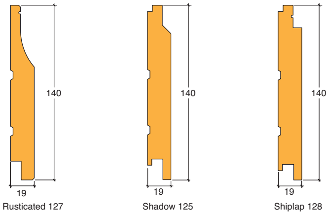
Figure 1: Pentarch Australian hardwood cladding profiles
