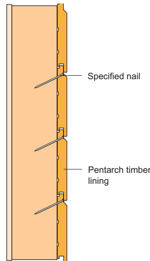
Figure 18: Secret fixing linings
