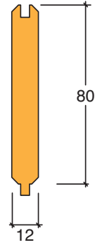
Figure 2: Pentarch Australian hardwood lining profiles
